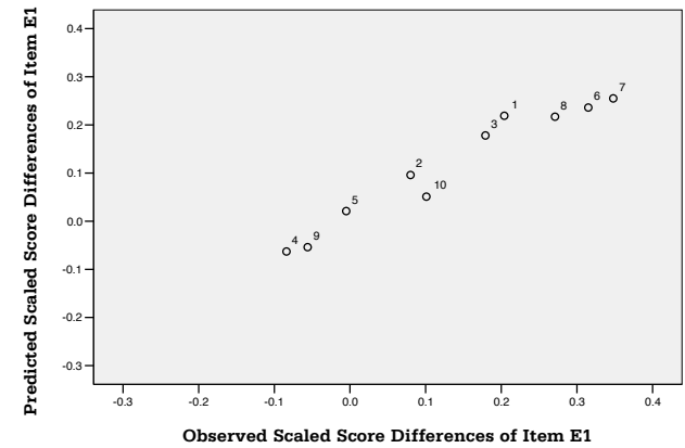
Figure 2. Scatterplot of predicted mean SSDs and observed mean SSDs after removing item E1.
